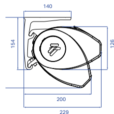
B50 S ceiling mounting
