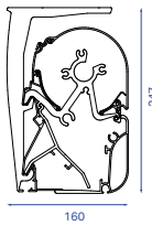
B25 ELITE / PRESTIGE ceiling mounting
