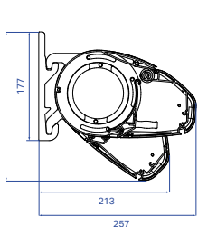
B50 XL wall mounting
