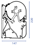
B25 ELITE / PRESTIGE wall mounting
