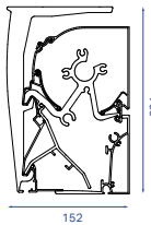
B27 ceiling mounting
