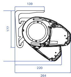
B50 XL ceiling mounting
