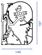
B25 wall mounting
