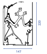
B27 ELITE / PRESTIGE wall mounting
