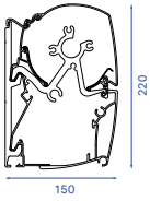
B24 ELITE / PRESTIGE wall mounting
