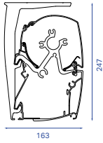
B24 ELITE / PRESTIGE ceiling mounting
